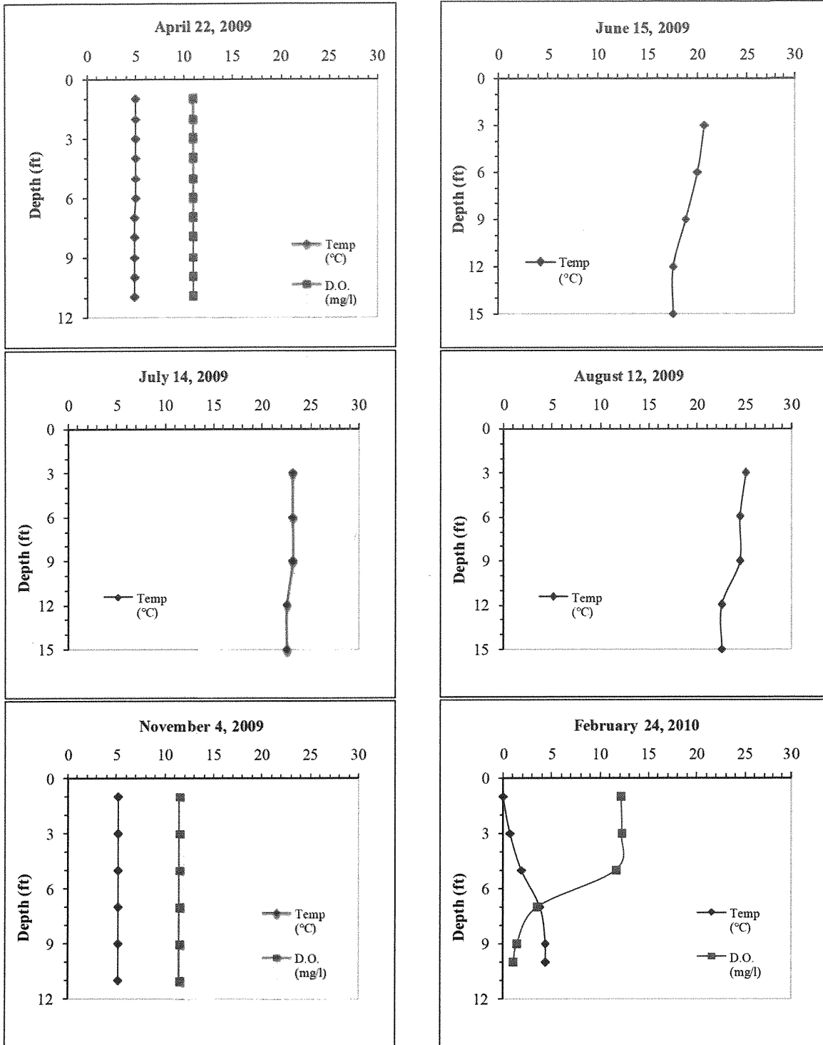
Figure 3.1-6. Pine Lake dissolved oxygen and temperature profiles.
