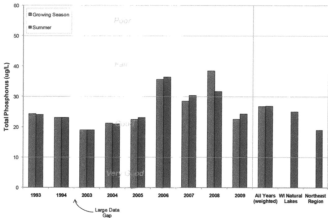
Figure 3.1-2. Pine Lake, regional, and state total phosphorus concentrations. Mean values calculated with summer month surface sample data. Water Quality Index values adapted from Lillie and Mason (1983).
